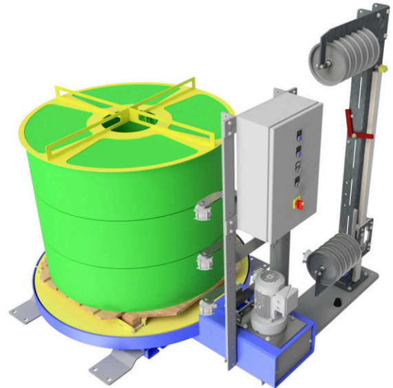
Strap accumulation system for plastic strap
